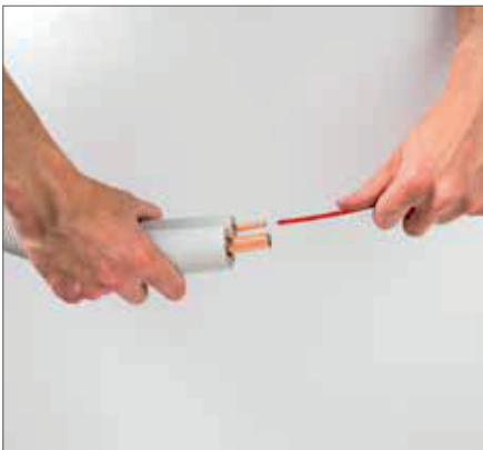
Step 1: Insert the flexible bender of the right diameter into the copper tube
